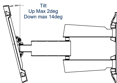
SIDE VIEW TILT ADJUSTMENT
