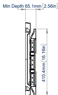
SIDE VIEW CLOSE TO THE WALL
