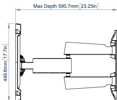
SIDE VIEW MAX EXTENSION
