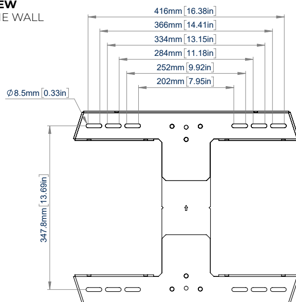
WALL PLATE
