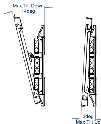
TILT ADJUSTMENT SIDE VIEW
