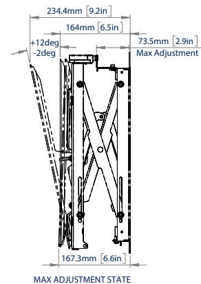
SIDE VIEW - CLOSED MAX ADJUSTMENT STATE
