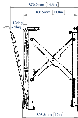
SIDE VIEW - OPEN STATE
