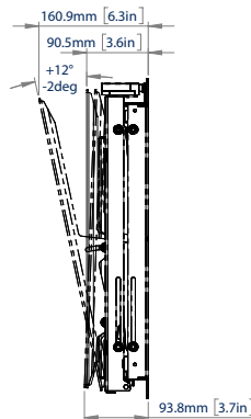
SIDE VIEW - CLOSED MIN ADJUSTMENT STATE
