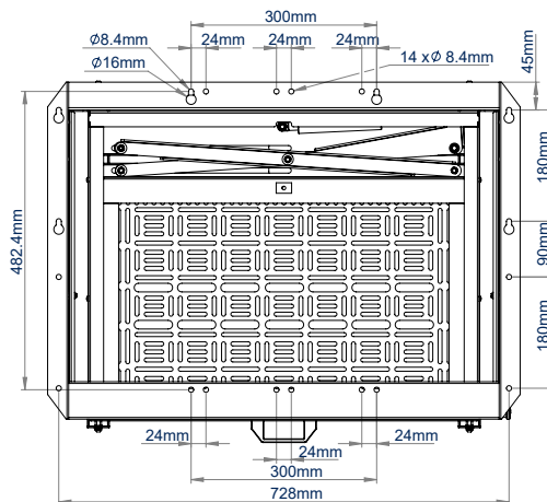
REAR VIEW
