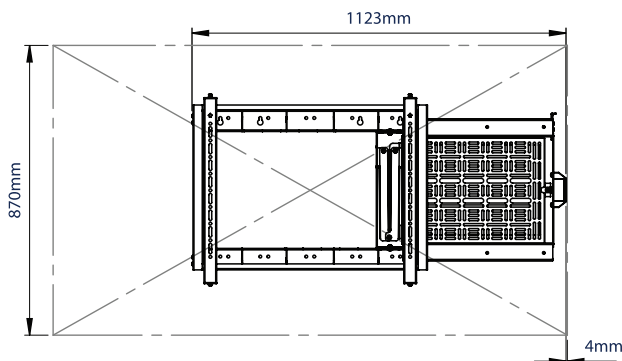
75" SCREEN CLOSED
