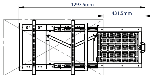
46" SCREEN OPEN
