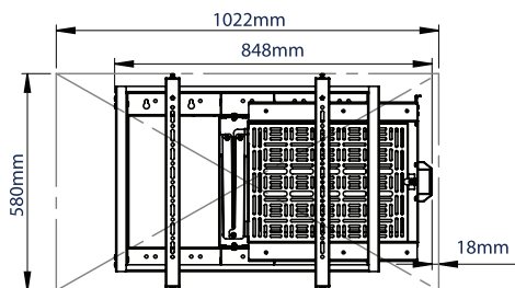
46" SCREEN CLOSED
