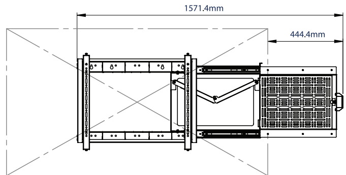
75" SCREEN OPEN
