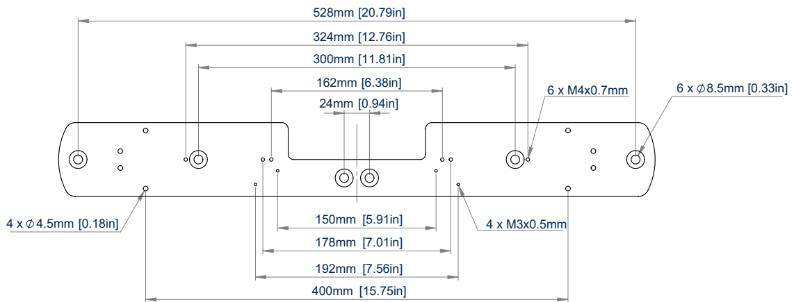
REAR VIEW
