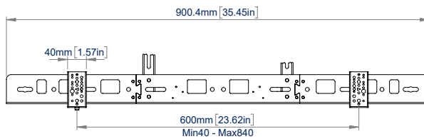
FRONT VIEW MOUNTING RAIL
