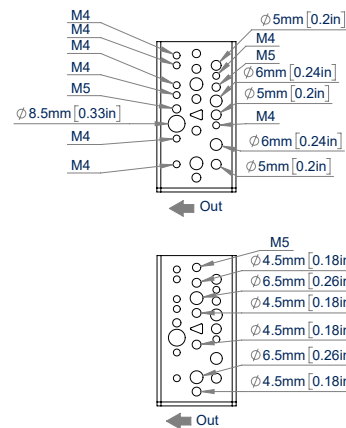
MOUNTING PLATE
