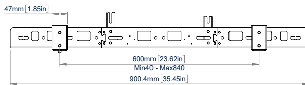
REAR VIEW MOUNTING RAIL
