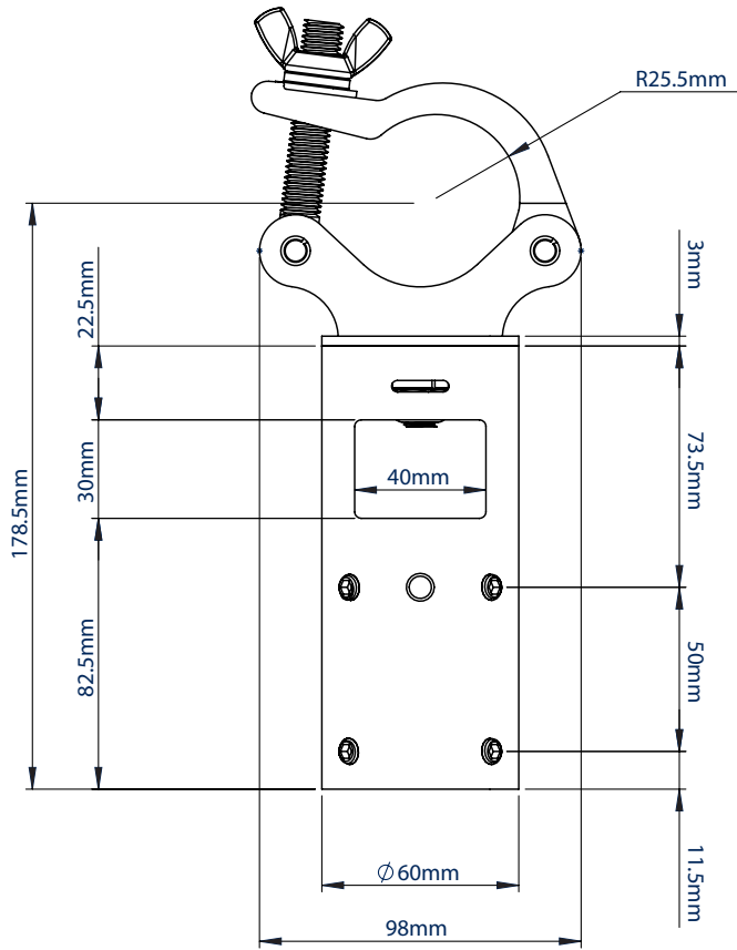
FRONT VIEW
