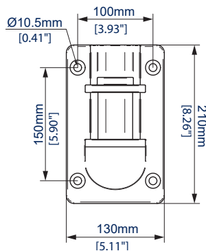
WALL PLATE
