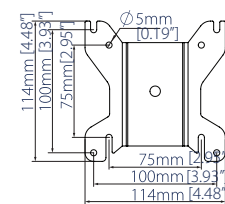
INTERFACE PLATE - FRONT VIEW
