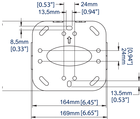
FRONT VIEW WALL PLATE
