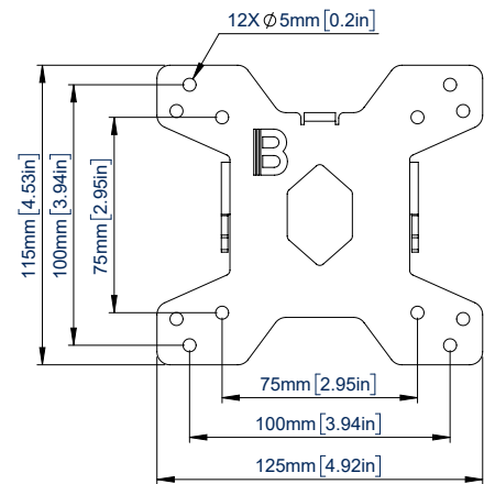
FRONT VIEW MOUNTING PLATE 100X100 OR 75X75
