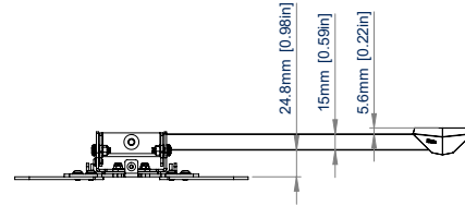
TOP VIEW FLAT TO WALL
