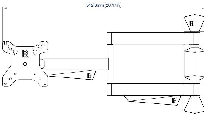
FRONT VIEW FLAT TO WALL
