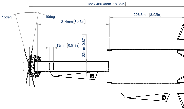
SIDE VIEW TILT ADJUSTMENT
