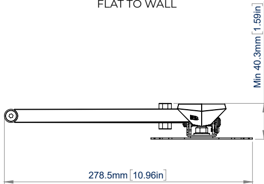
TOP VIEW FLAT TO WALL
