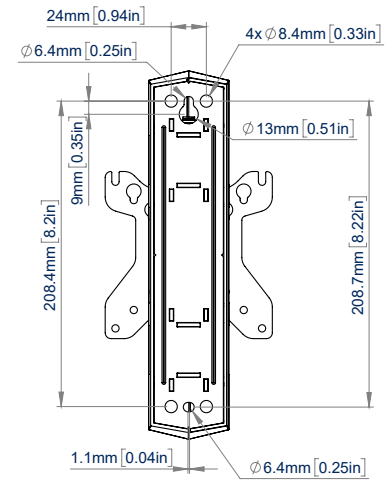
REAR VIEW WALL PLATE
