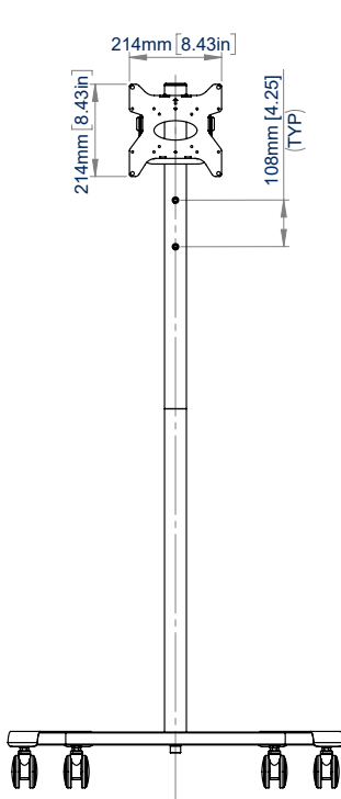
FRONT VIEW
