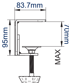
DESK CLAMP
