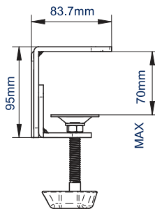
DESK CLAMP
