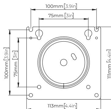
Wall Plate
