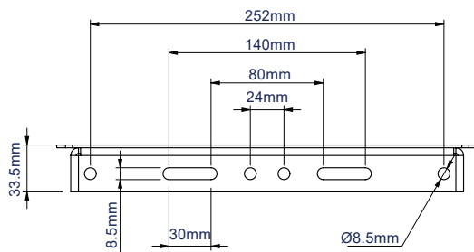
BACK VIEW
