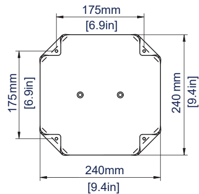
BASE PLATE
