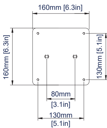
TOP PLATE
