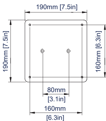
TOP PLATE
