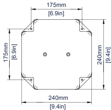
BASE PLATE
