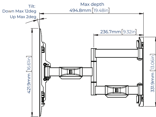
SIDE VIEW WITH EXTENSION
