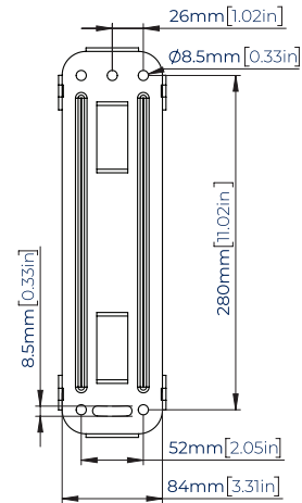
WALL PLATE
