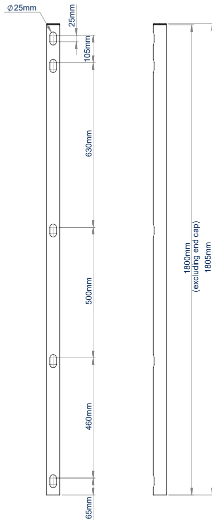
REAR VIEW
