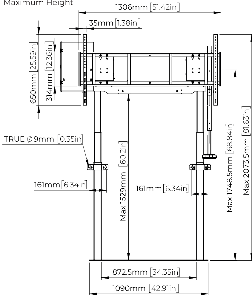
Front View Maximum Height
