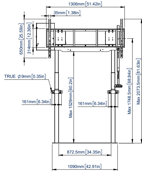
FRONT VIEW MAX EXTENSION
