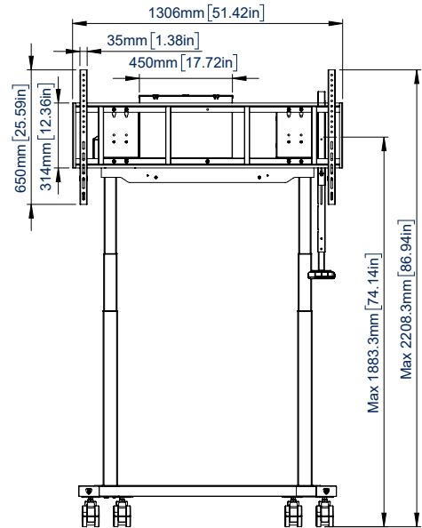
FRONT VIEW MAX EXTENSION
