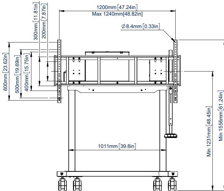
FRONT VIEW MIN EXTENSION
