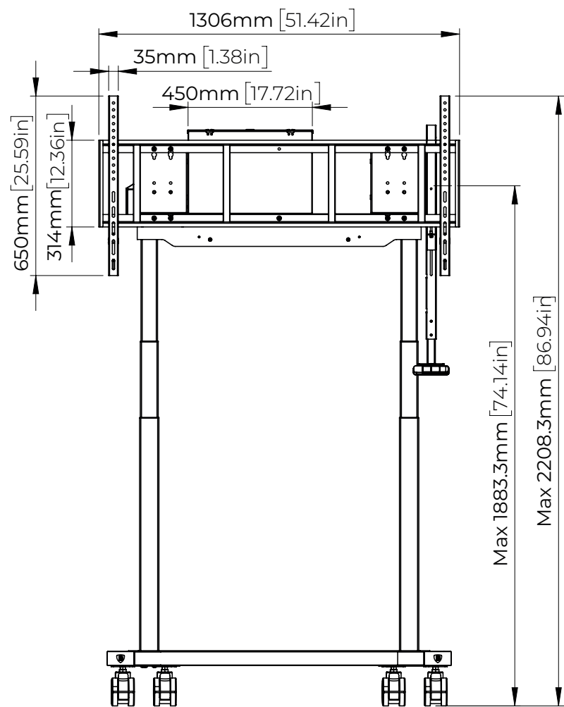
Front View Maximum Height
