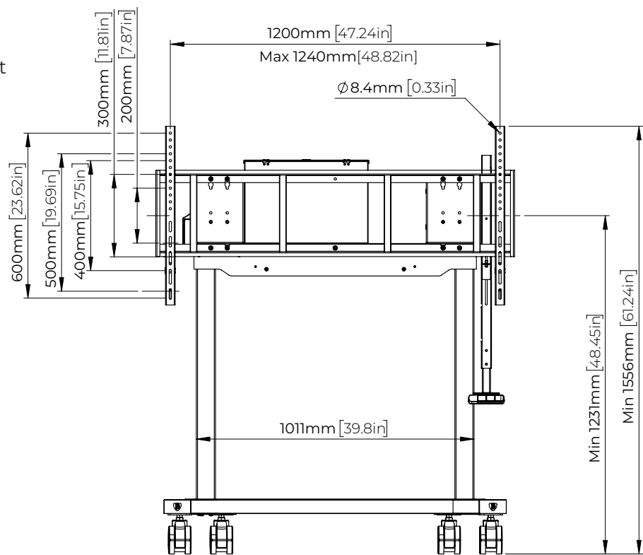
Front View Minimum Height
