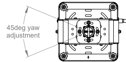
PROJECTOR MOUNT TOP VIEW
