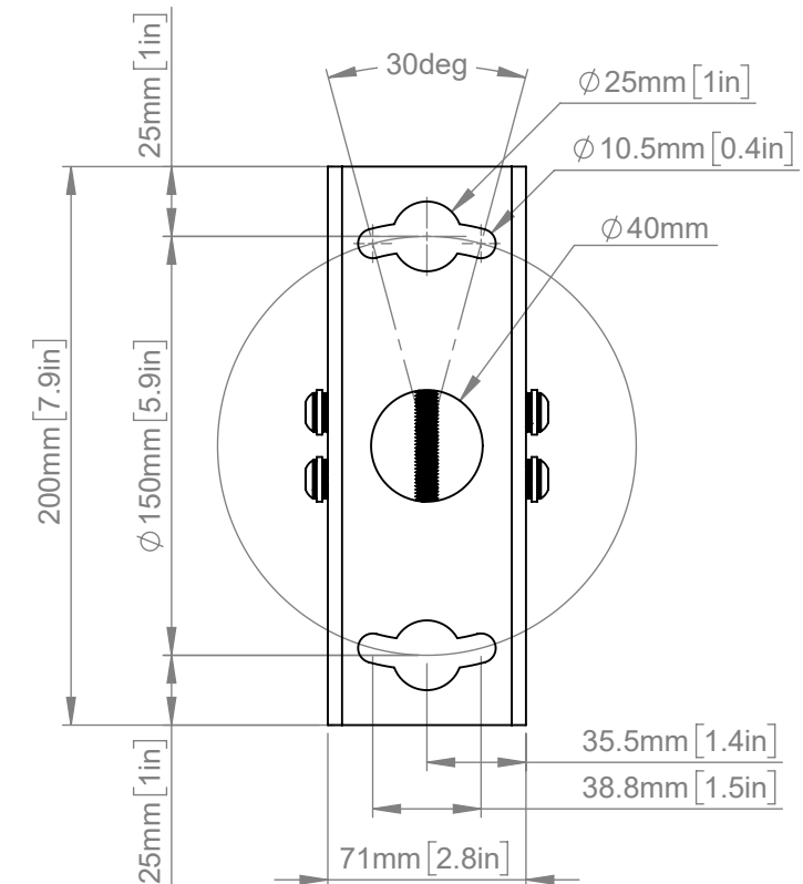
TOP VIEW OF CEILING PLATE SCALE 1 : 3
