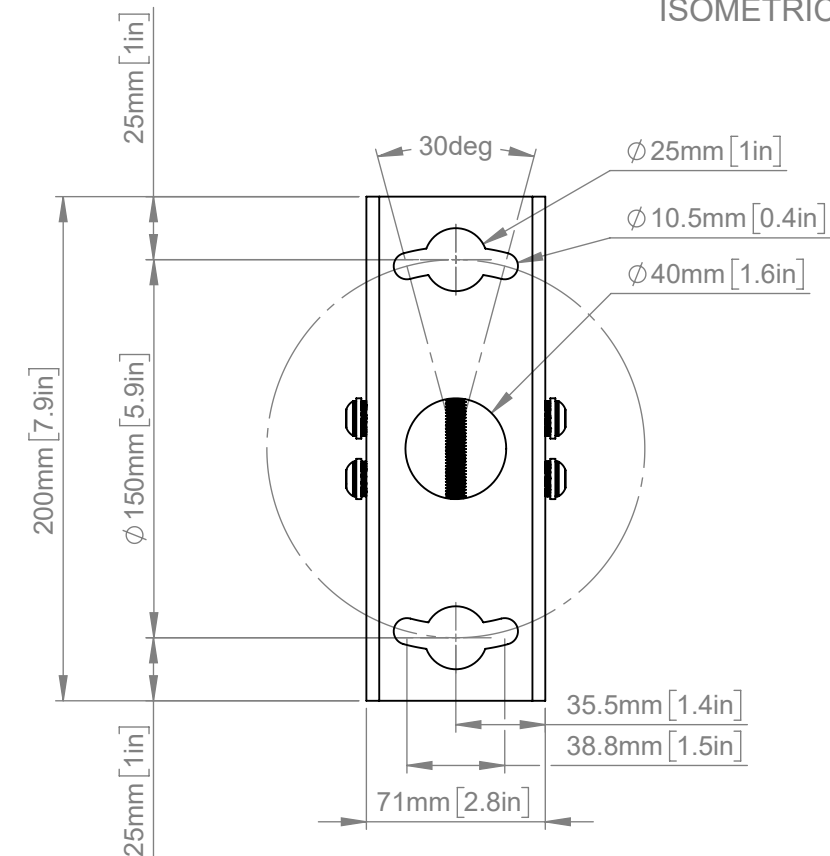
TOP VIEW OF CEILING PLATE SCALE 1 : 3
