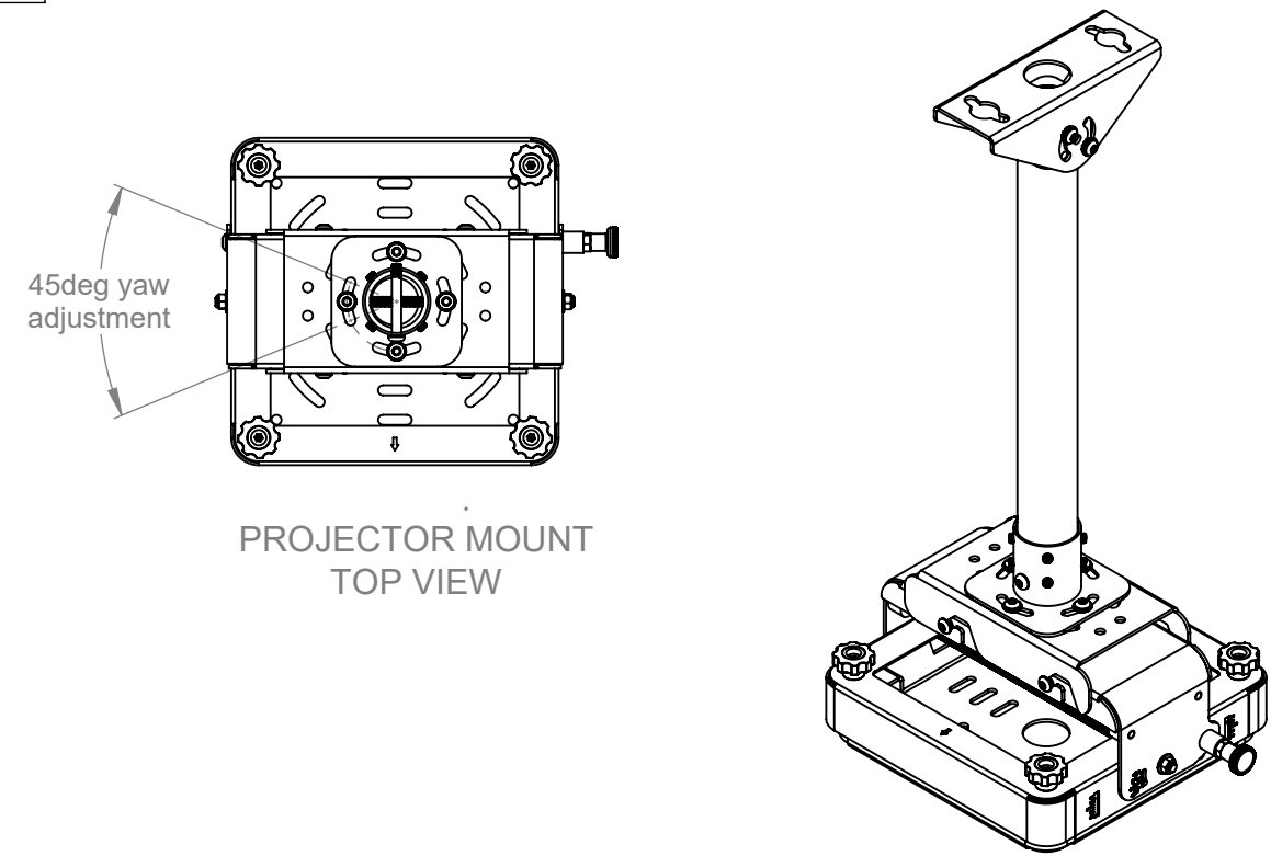
ISOMETRIC VIEW
