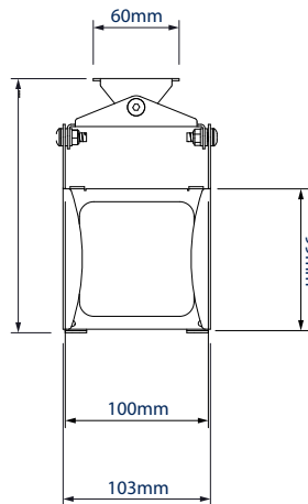
TOP VIEW WITH SWIVEL
