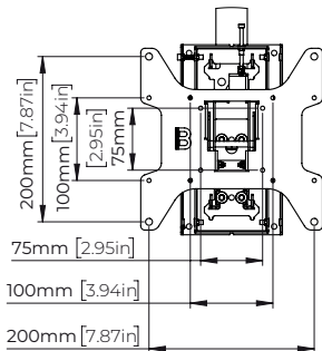
Front View - Interface Plate
