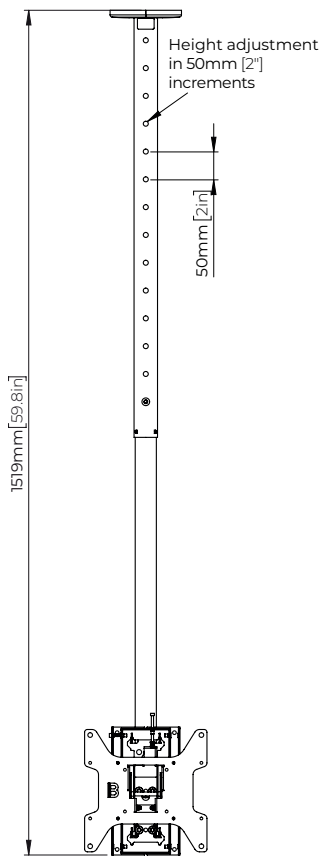
Front View - Interface Plate
