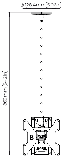
Front View - Min. Extension
