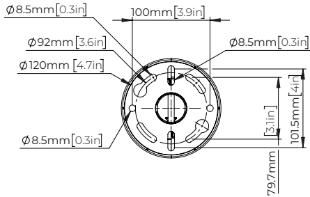
Top View - Ceiling Plate
