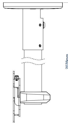
BT5970-FD200 SIDE VIEW
