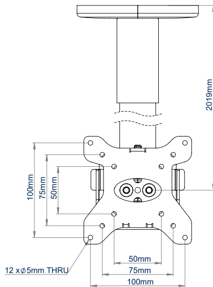
BT5970-FD200 FRONT VIEW
