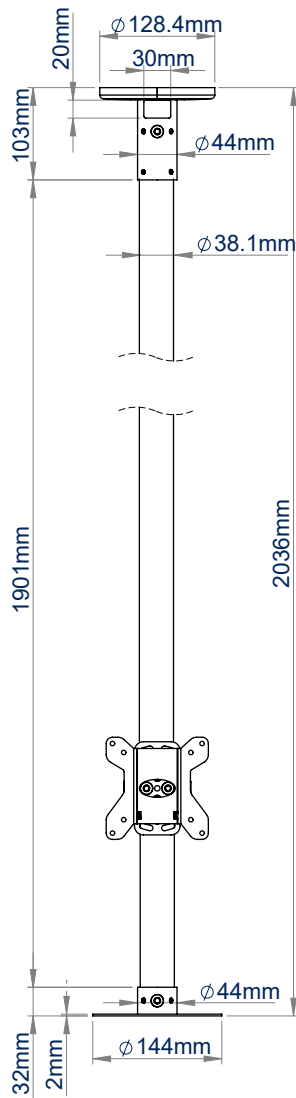
BT5963-FD200 FRONT VIEW
