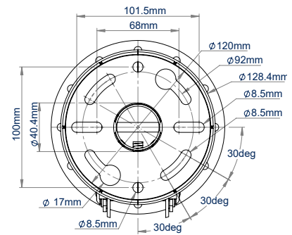
CEILING PLATE TOP VIEW
