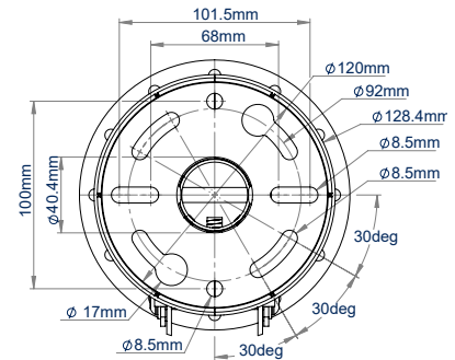
CEILING PLATE TOP VIEW
