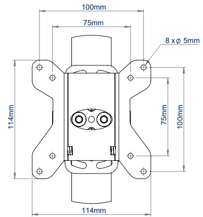
SCREEN MOUNT FRONT VIEW
