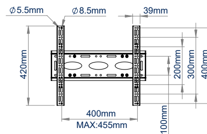
MOUNT
