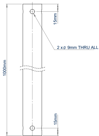
SIDE VIEW 1 METRE
