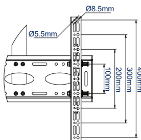
INTERFACE-ARM CLOSE-UP
