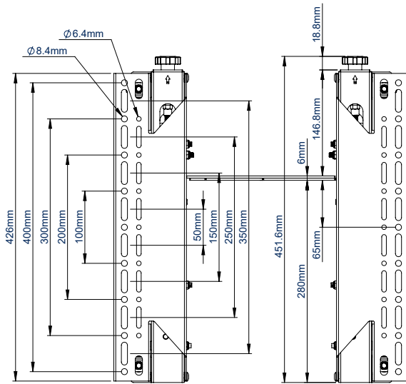
VISTA FRONTAL
