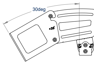
TILT 30 DEGREE
