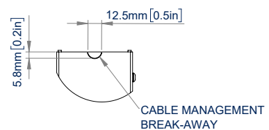
DETAIL A SCALE 1 : 3
