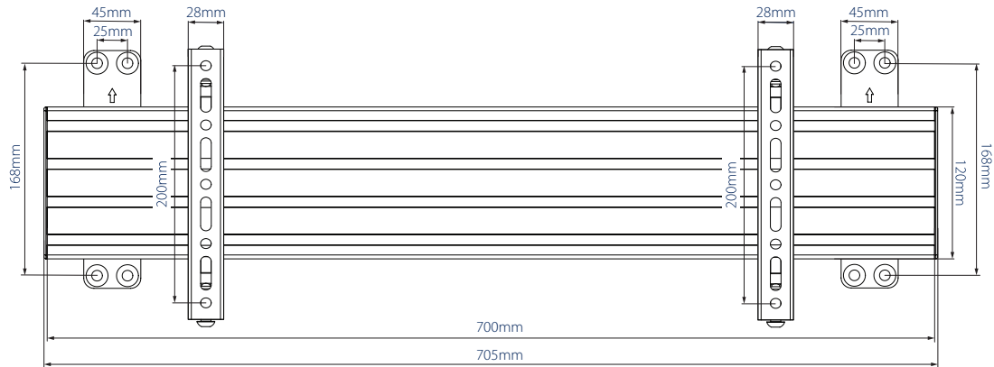
VISTA FRONTAL
