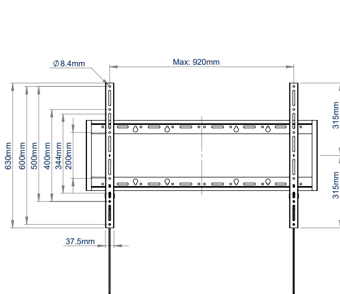
VISTA FRONTAL
