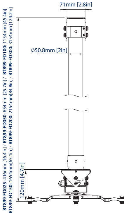
VISTA FRONTAL
