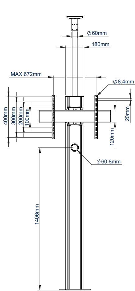
VISTA FRONTAL
