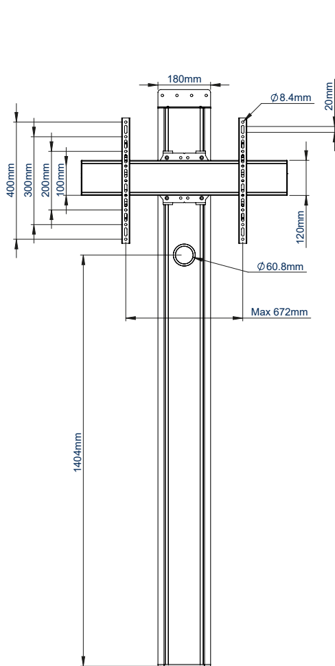
VISTA FRONTAL
