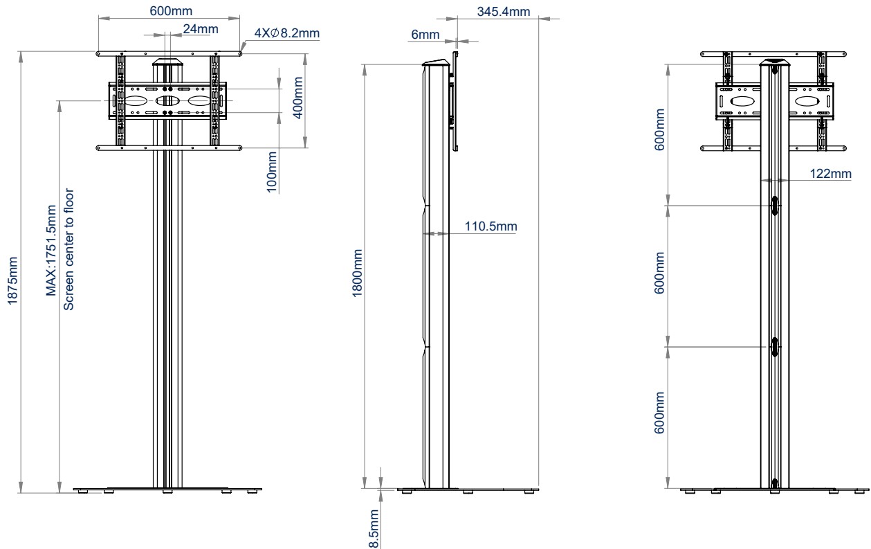
VISTA FRONTAL
