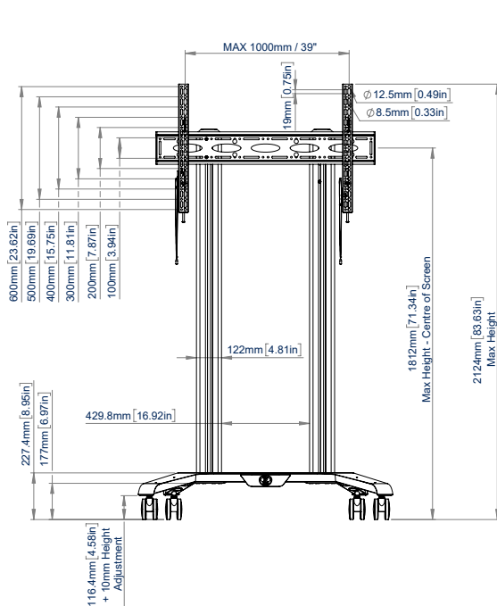
VISTA FRONTAL
