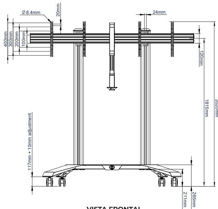
VISTA FRONTAL
