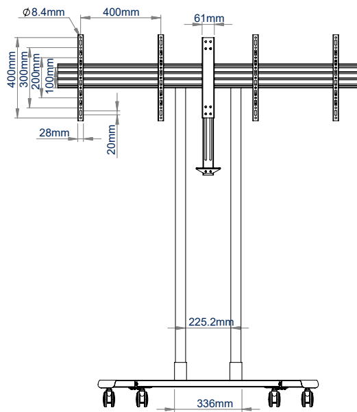
VISTA FRONTAL
